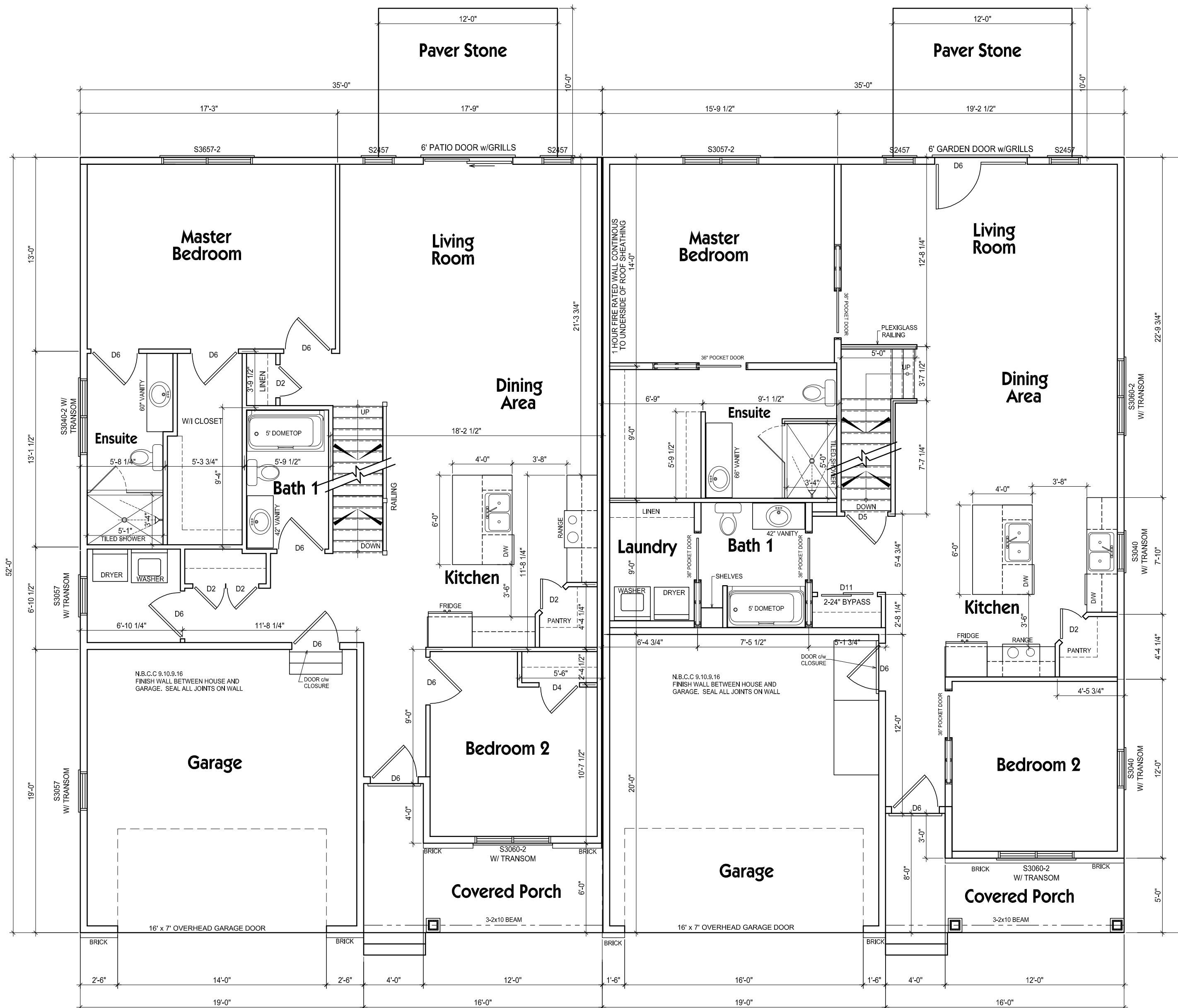
Unit 1 Floor Plan FIRST FLOOR AREA: 1351 sq.ft. GARAGE AREA: 408 sq.ft.
